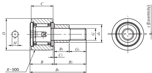
CFE ... BR Outside diameter of eccentric collar d_e 9-13mm
